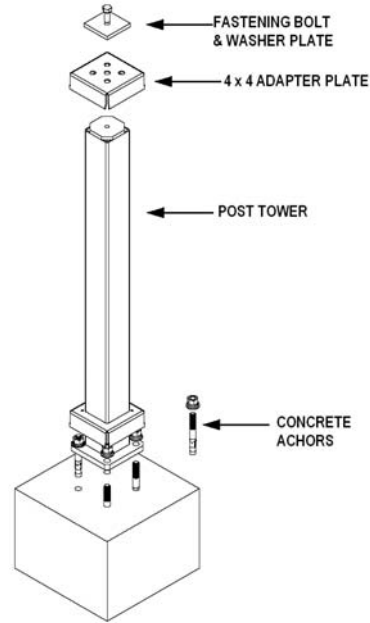
Post Tower on Concrete Decks
