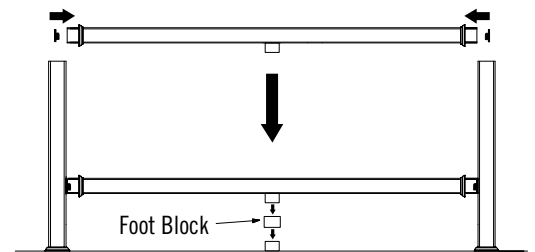
Install Bottom Rail
