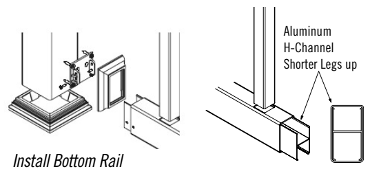
Install Bottom Rail
